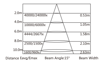
ILUMINANCE AT DISTANCE
