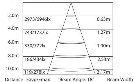
Illuminance at Distance
