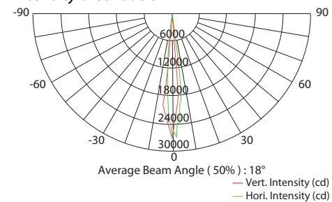
Intensity Distribution
